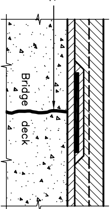
JOINT OR ACTIVE WIDE CRACK IN BRIDGE DECK
