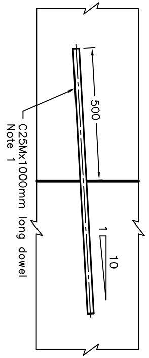
DOWEL CONNECTION DETAIL TYPE II
