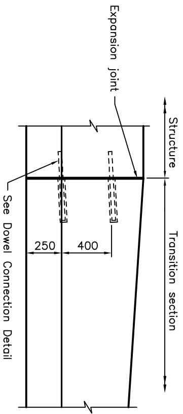
DOWEL CONNECTION WITH EXPANSION JOINT TYPE I
