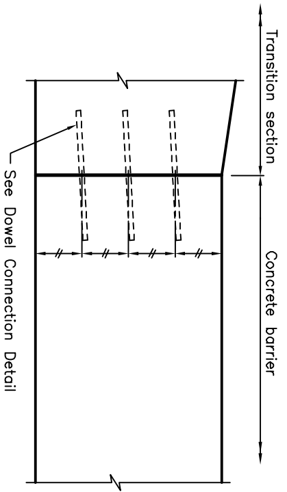
DOWEL CONNECTION WITHOUT EXPANSION JOINT TYPE II
