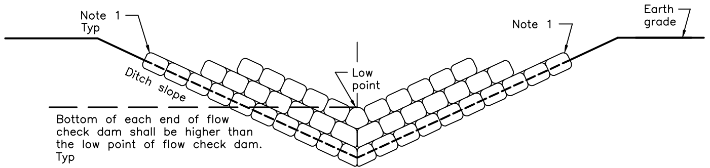
SECTION A-A FLAT BOTTOM DITCH
