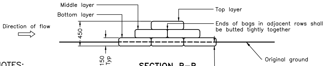
SECTION B-B
