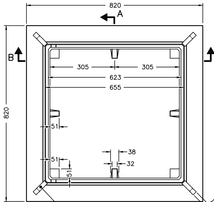
FRAME PLAN
