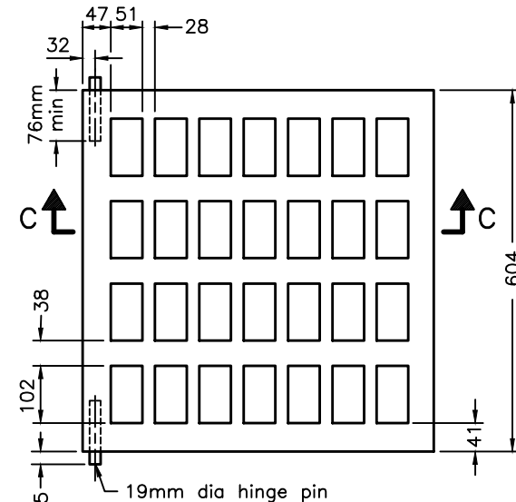
GRATE PLAN
