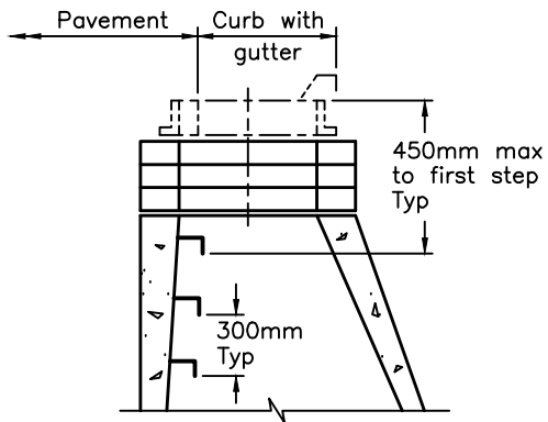
SECTION THROUGH TAPER TOP
