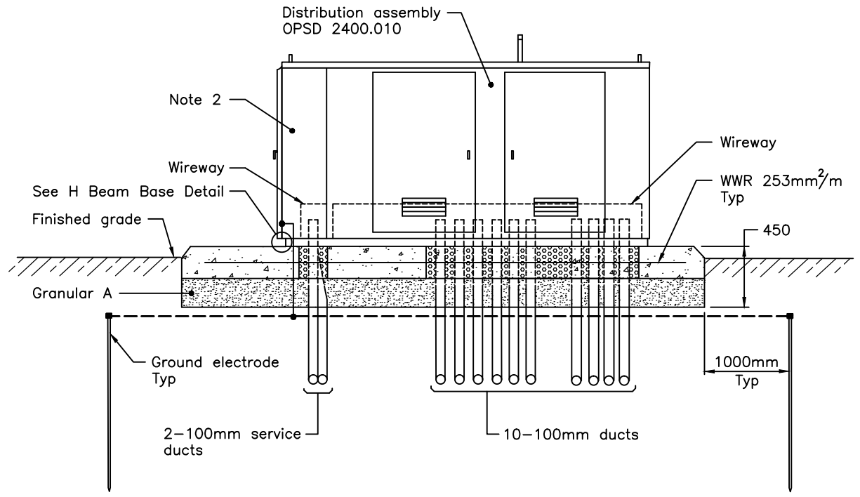
SECTION B-B
