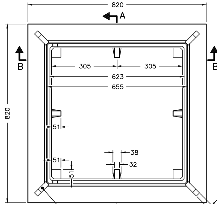
FRAME PLAN
