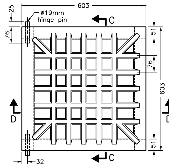
GRATE PLAN
