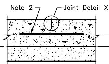
LONGITUDINAL JOINT MULTI-LANE PAVING
