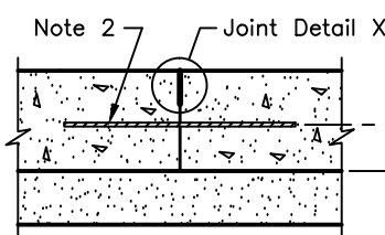
LONGITUDINAL JOINT SINGLE LANE PAVING
