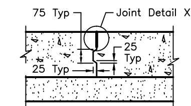
LONGITUDINAL KEYWAY JOINT WITHOUT TIE BAR
