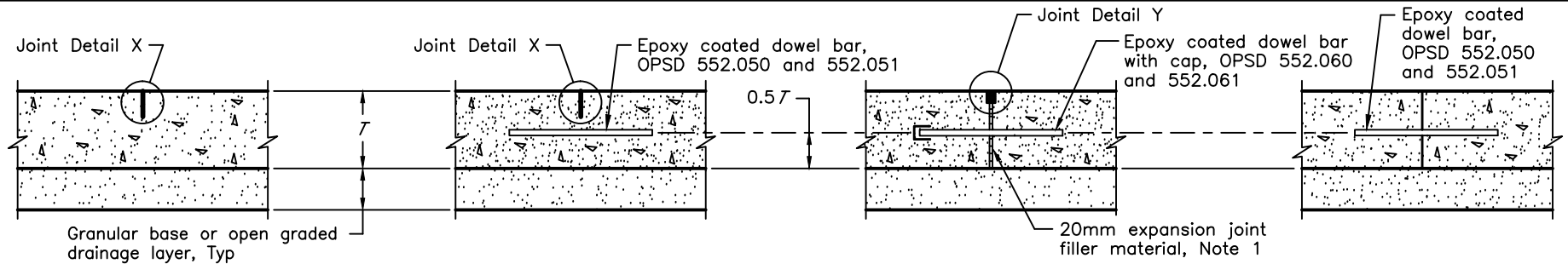
CONTRACTION JOINT WITHOUT DOWEL BAR
