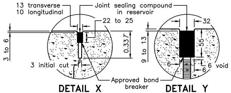
JOINT DETAILS RESERVOIR CUT TYPE
