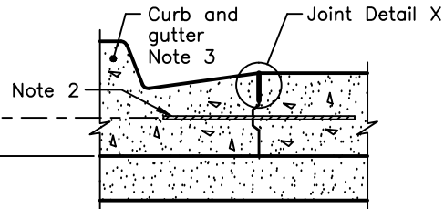
LONGITUDINAL JOINT CONCRETE SLAB ADJACENT TO CURB WITH GUTTER
