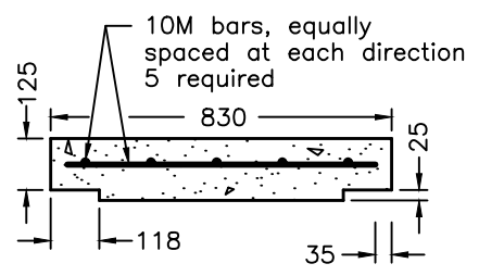
CAP DETAIL
