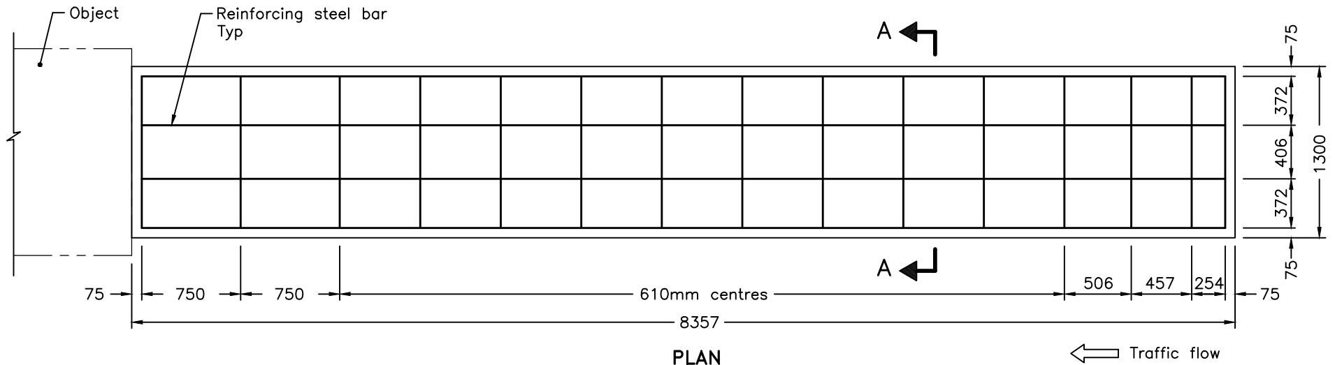
PLAN CONCRETE PAD FOR TL-3 SYSTEM CONFIGURATION
