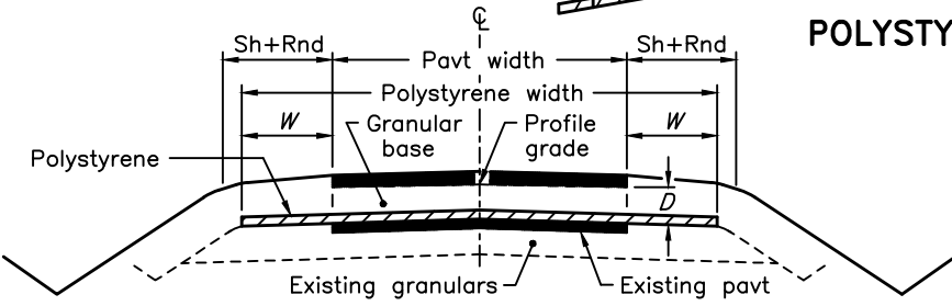
TRANSVERSE GRADE RAISE SECTION
