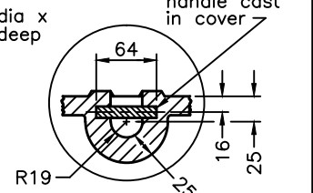
BAR HANDLE DETAIL
